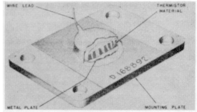
Figure 2-24. Disc Thermistor
