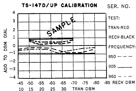
Figure 4-2. Typical Calibration Chart
