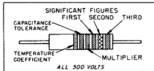
RMA COLOR CODE FOR TUBULAR CERAMIC-DIELECTRIC CAPACITORS
