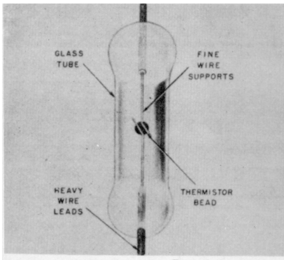
Figure 2-23. Bead Thermistor
