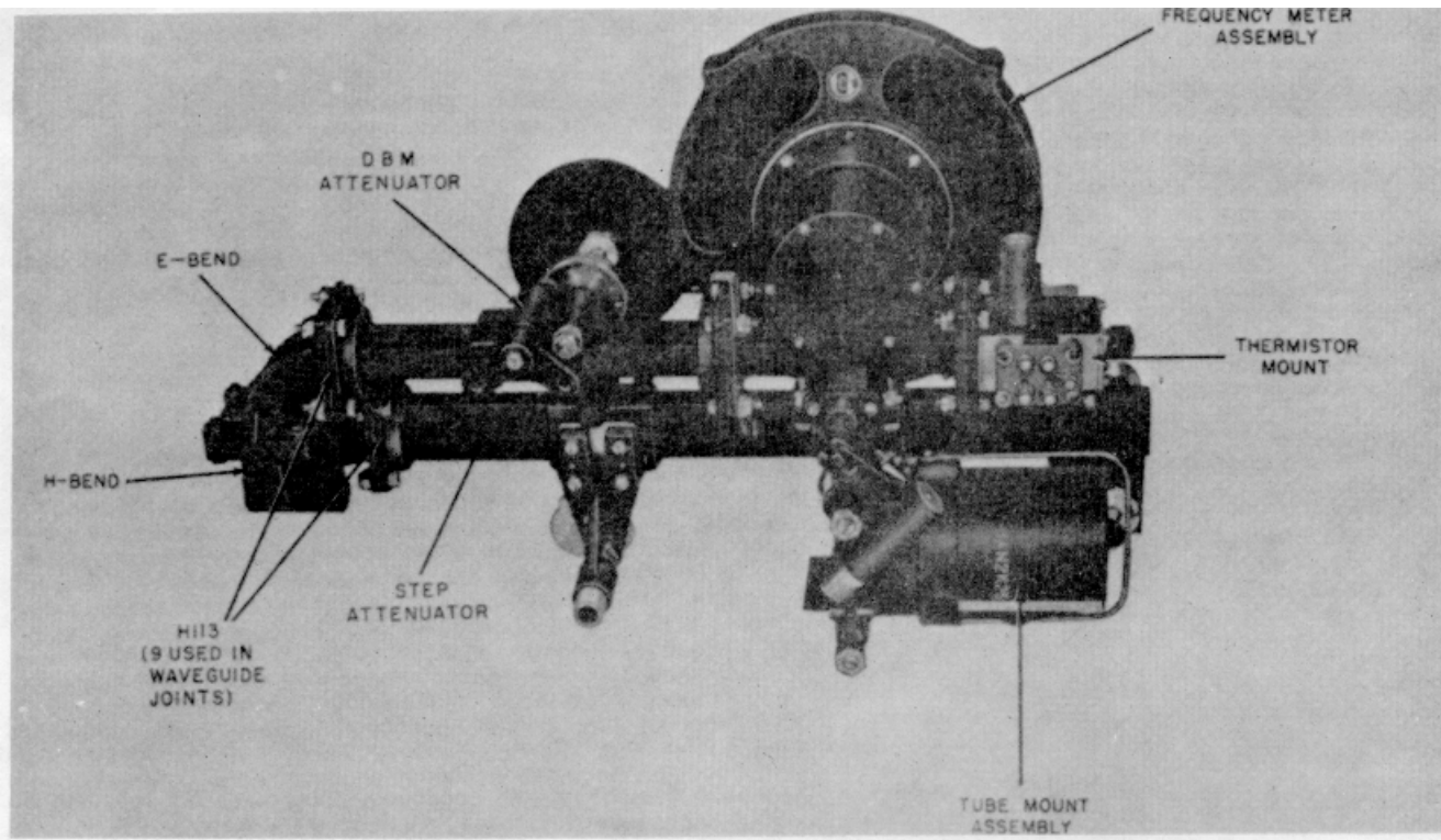
Figure 5-6. Assembled Wave Guide, Rear View
