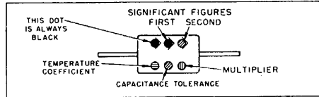
JAN 6-DOT COLOR CODE FOR MICA-DIELECTRIC CAPACITORS
