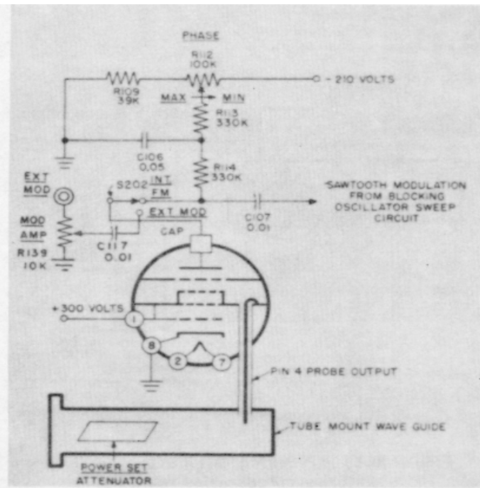
Figure 2-19. Test Oscillator Circuit
