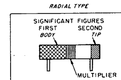
JAN COLOR CODE FOR FIXED COMPOSITION RESISTORS
