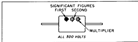
RMA 3-DOT COLOR CODE FOR MICA-DIELECTRIC CAPACITORS
