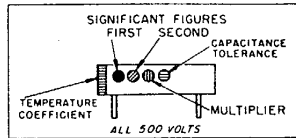
JAN COLOR CODE FOR FIXED CERAMIC-DIELECTRIC CAPACITORS RADIAL TYPE NON-INSULATED AXIAL TYPE INSULATED
