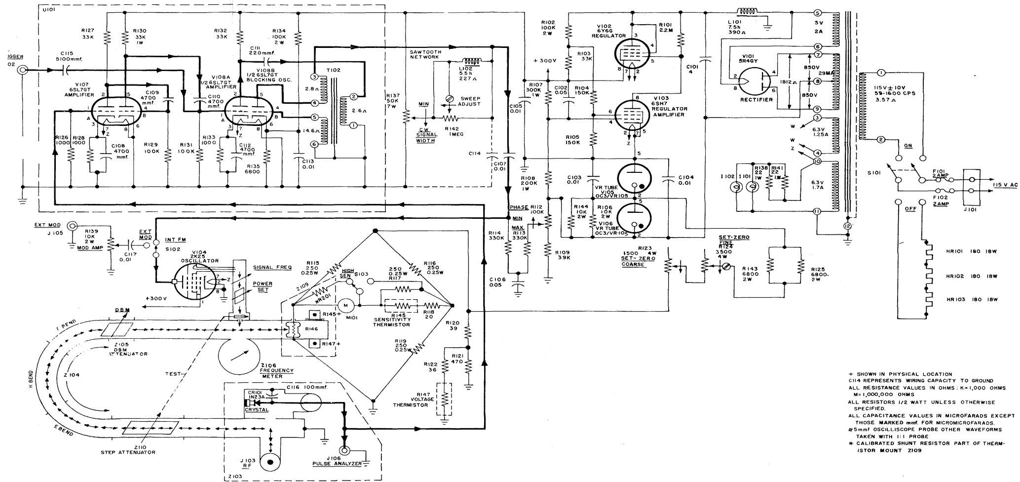
Figure 5-16. Test Set TS-147D/UP Complete System Schematic
