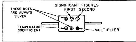
JAN 6-DOT COLOR CODE FOR PAPER-DIELECTRIC CAPACITORS
