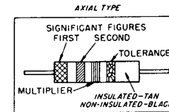
RMA COLOR CODE FOR FIXED COMPOSITION RESISTORS
